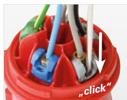
3) Re-open terminal
